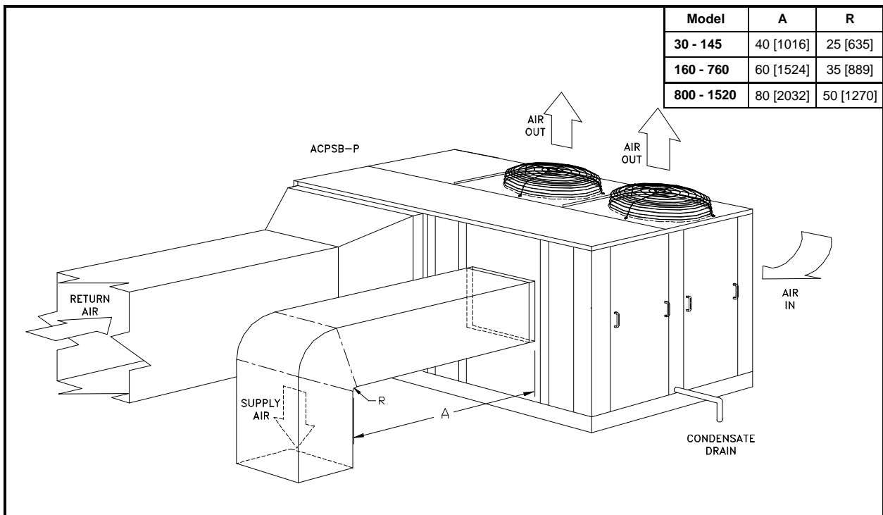
FIGURE 3.4: SUGGESTED METHOD FOR CONNECTING SUPPLY DUCT
