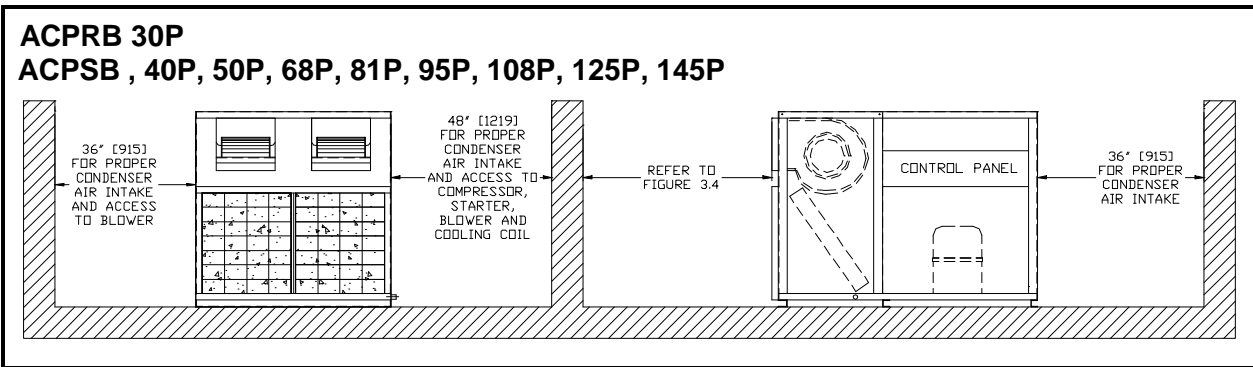
FIGURE 3.3 AIR COOLED SINGLE PACKAGE AIR CONDITIONER CLEARANCE
