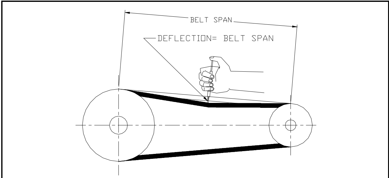
Figure 5.4: Belt Span
